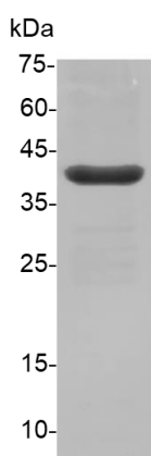
SDS-PAGE analysis of Recombinant Bla g 9 protein
