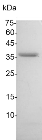
SDS-PAGE analysis of Recombinant Bla g 7 protein
