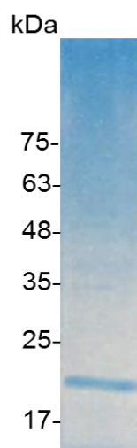
SDS-PAGE analysis of recombinant human IL-21
