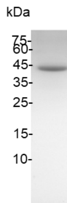
SDS-PAGE analysis of Gal d 2 protein
