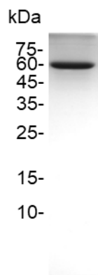
SDS-PAGE analysis of Bos d 6 protein
