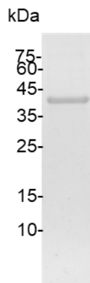
SDS-PAGE analysis of Recombinant Gal d 2 protein
